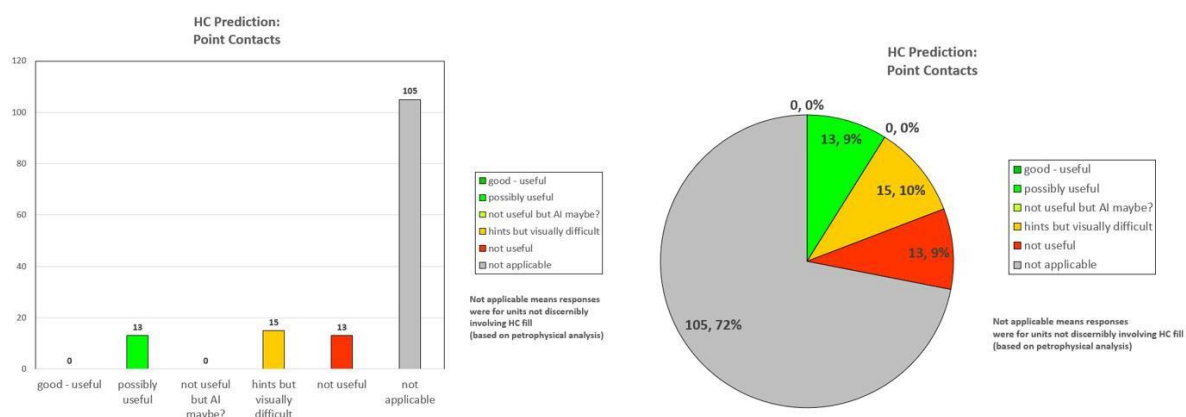
Figure 18: There are not a large number of thick very strong saturation in the wells studied, nevertheless where some HC saturation was perceived by petrophysical analysis, about a third of these showed some manifestation in the ADR curves.
